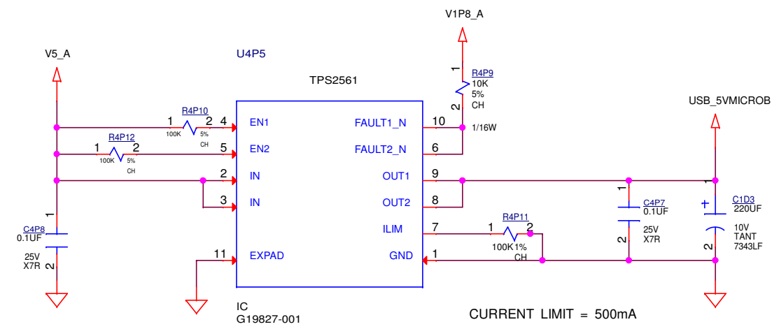
MICRO USB2.0 PORT 1
